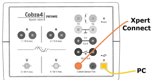
Fig. 4: Cobra4 Xpert-Link
